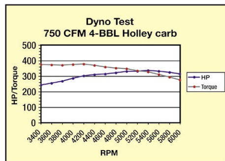
Peak HP: 337 @ 5400 rpm
