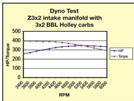
Peak HP: 346 @ 5200 rpm
